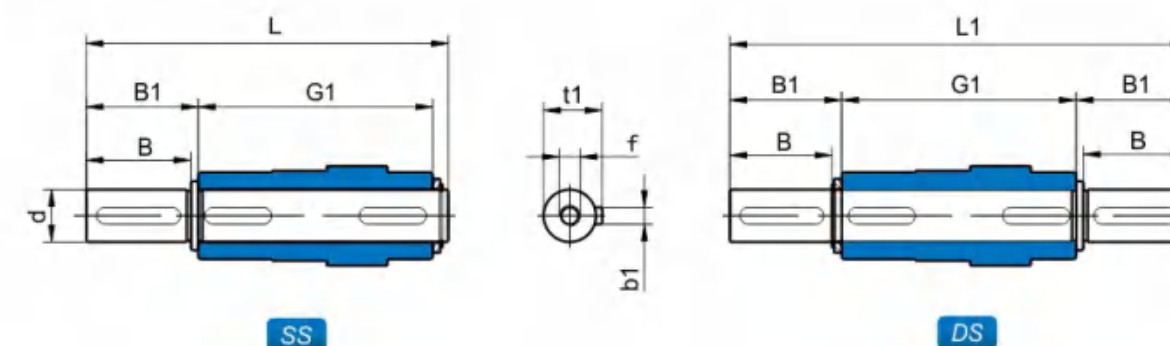
输出轴 / Output Shafts
