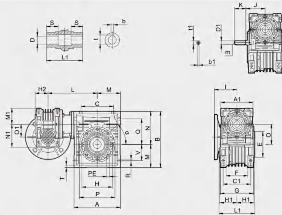
DRV外形尺寸 / DRV Outline Dimension
