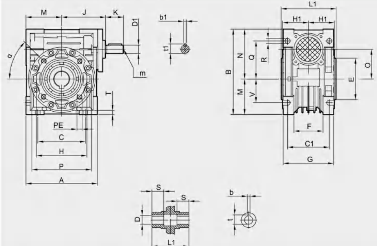
NRV外形尺寸 / NRV Outline Dimension
